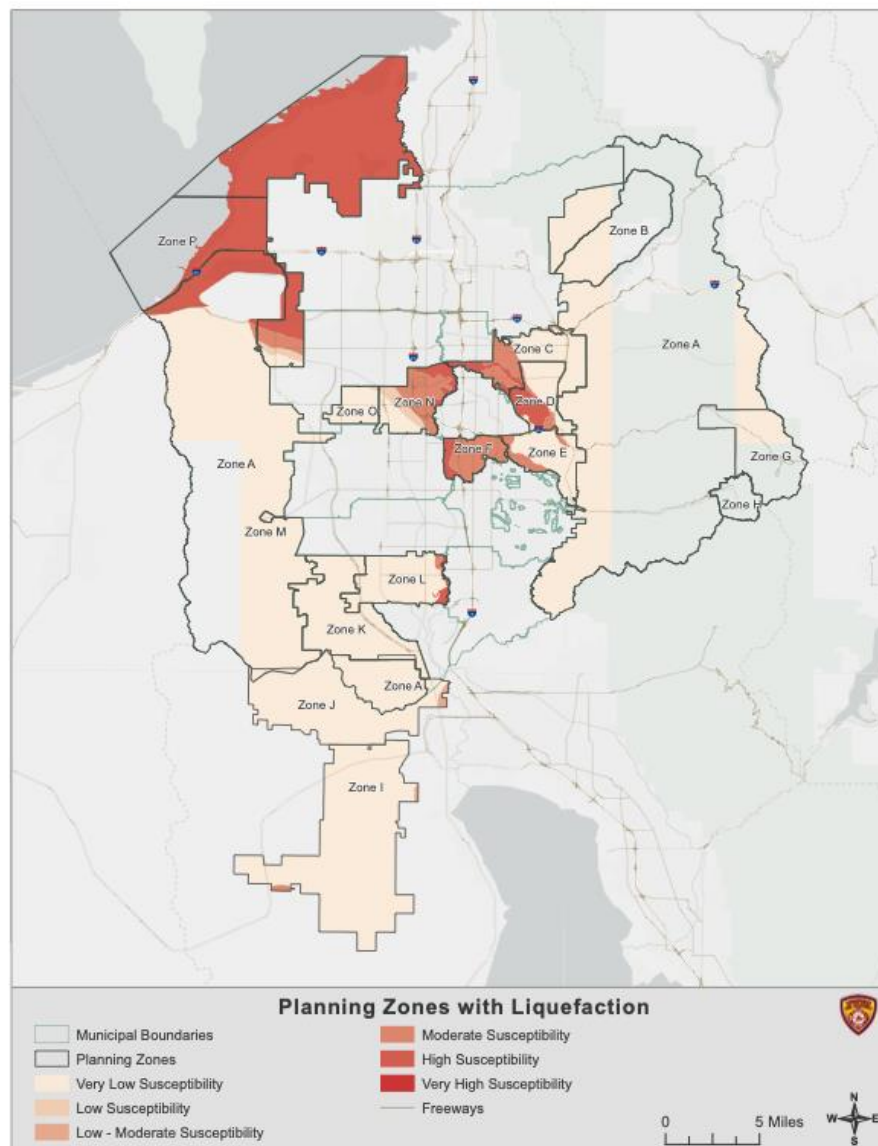
Map 10 - Liquefaction Areas
