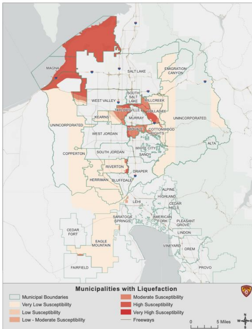
Map 57 - Liquefaction Areas
